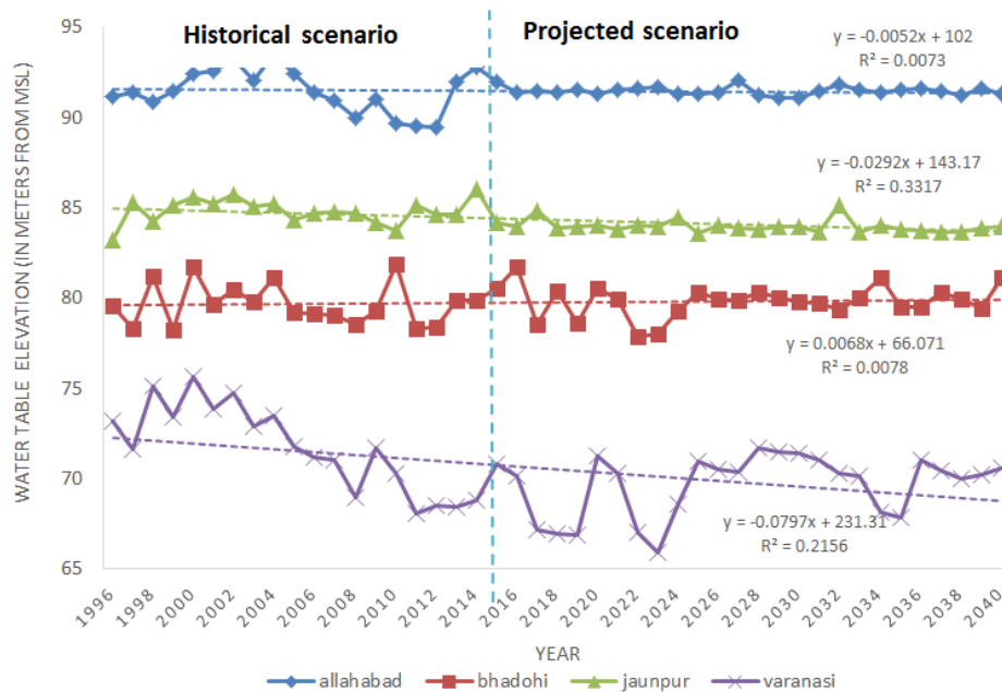
Figure 4: The water table elevation (meters) from mean sea level against the years (1996-2040) for historical and predicted scenario
